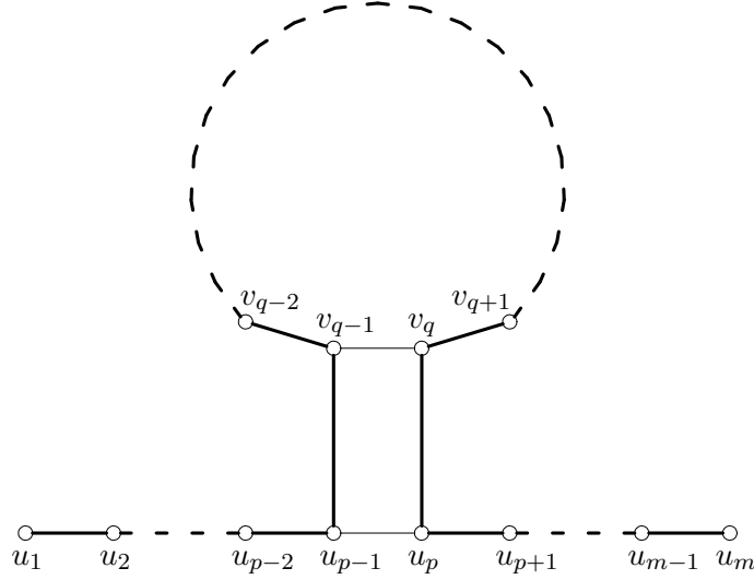
Figure 1: The path used to prove (5).
